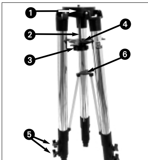
Fig. 3: Field Tripod. (1) Tripod Head; (2) Threaded Rod; (3) Tension Knob; (4) Spreader Bar; (5) Lock Knobs;
